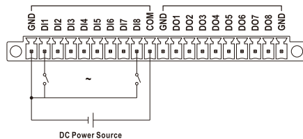
Dry contact wiring diagram
