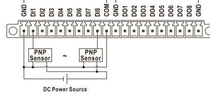
Wet contact Sink PNP wiring diagram
