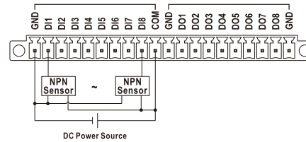
Wet contact Source (NPN) wiring diagram
